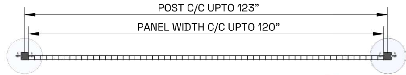
TOP VIEW
