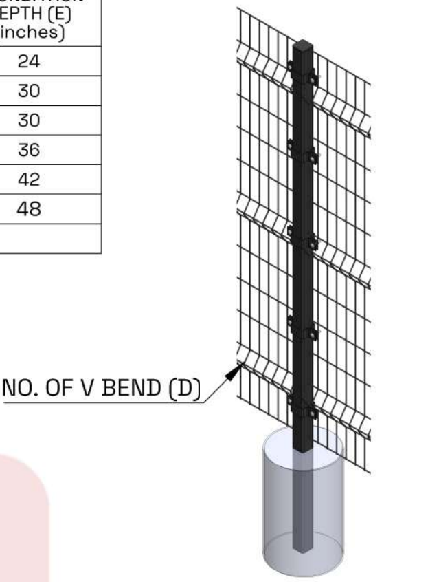
ISOMETRIC VIEW
